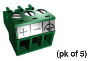
DC Power Connector Part No. EA-MG-DC-CON
