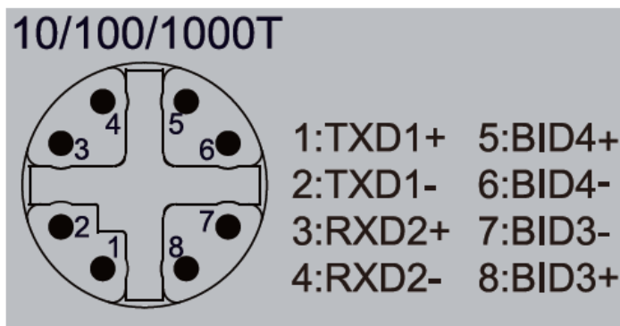
Switch connector
