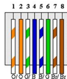
Pin assignment of M12 10/100/1000T network connector
