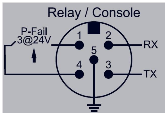
Pin assignment of alarm relay
