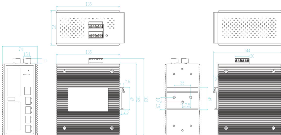
24V model
